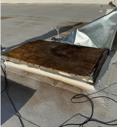
Metal Cap Repair
